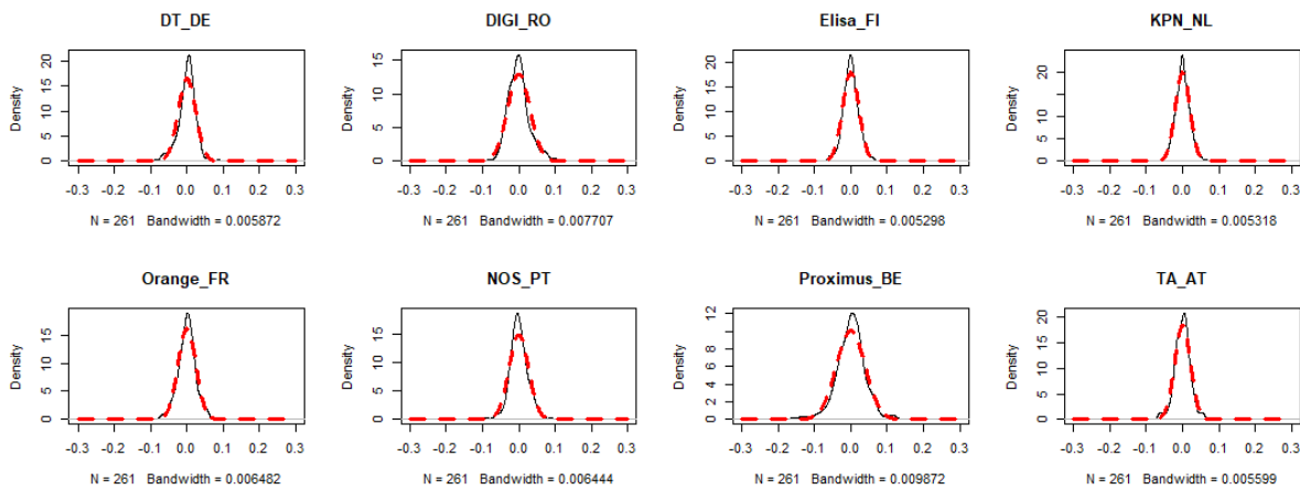
Figure A3 – Density plot of the residual of the distribution
